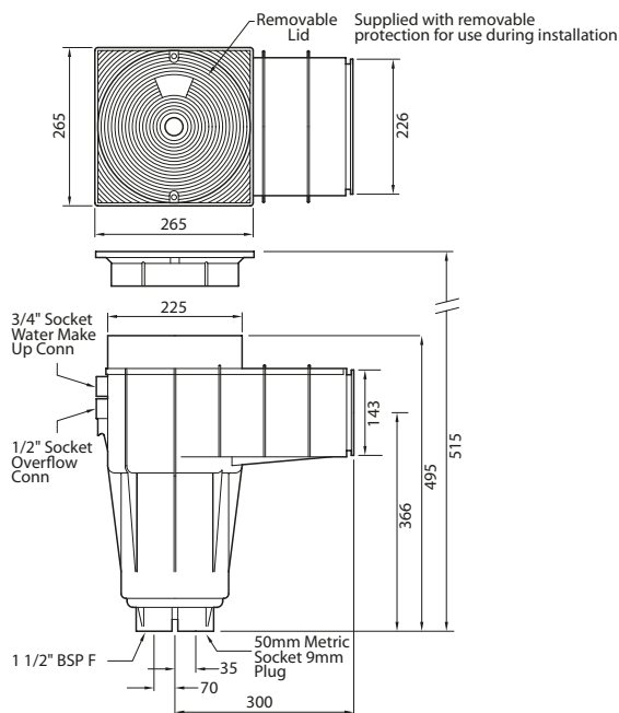
HD100SN (conc/collar) HD100LAK (liner adapt kit) Has adjustable flow restrictor for bottom connection. Either flap or collar weir
