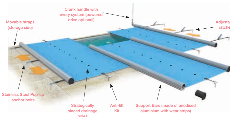
Quick release system as standard with Evolution models
