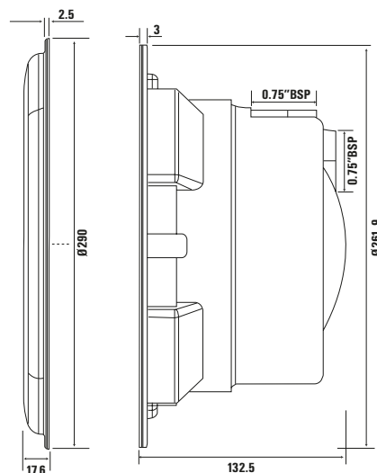
Niche & fascia ring
