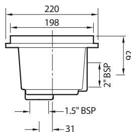
16,818mm² open surface area HD33D
