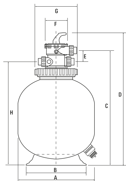
Top Mount
