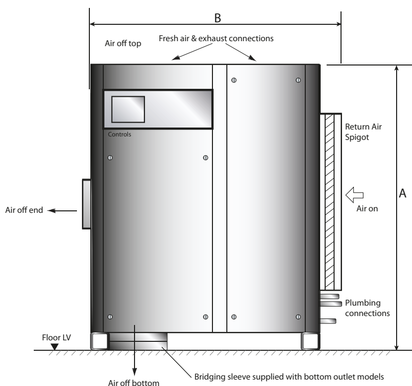
Front View Delta 1-12 – (mirror image versions available on Delta 4 and above)
