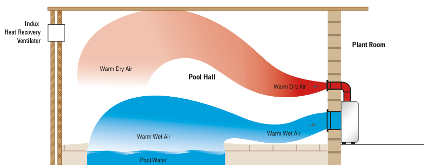
Through-The-Wall Model
