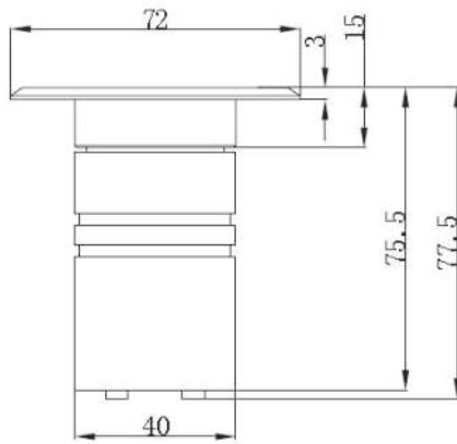
PU2 Concrete Pool Lights
