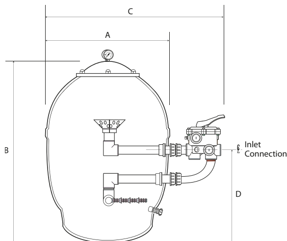
Side Mount
