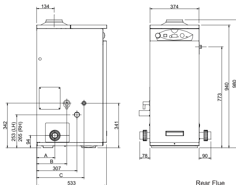
Rear Flue
