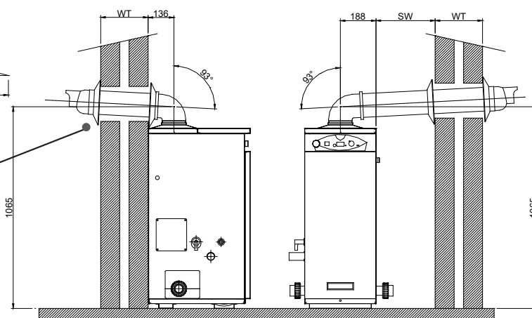
Left/Right Flue
