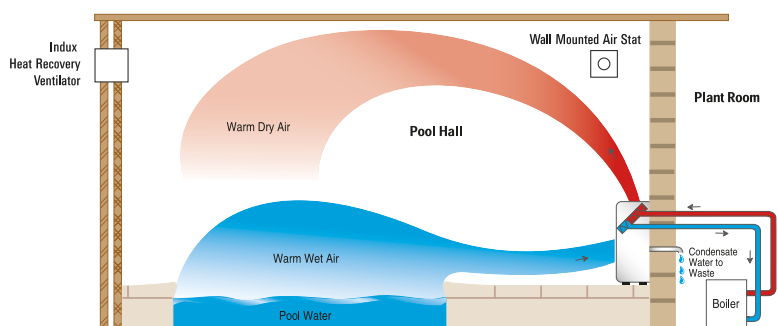
Standard Model Shown With Air Heating Facility
