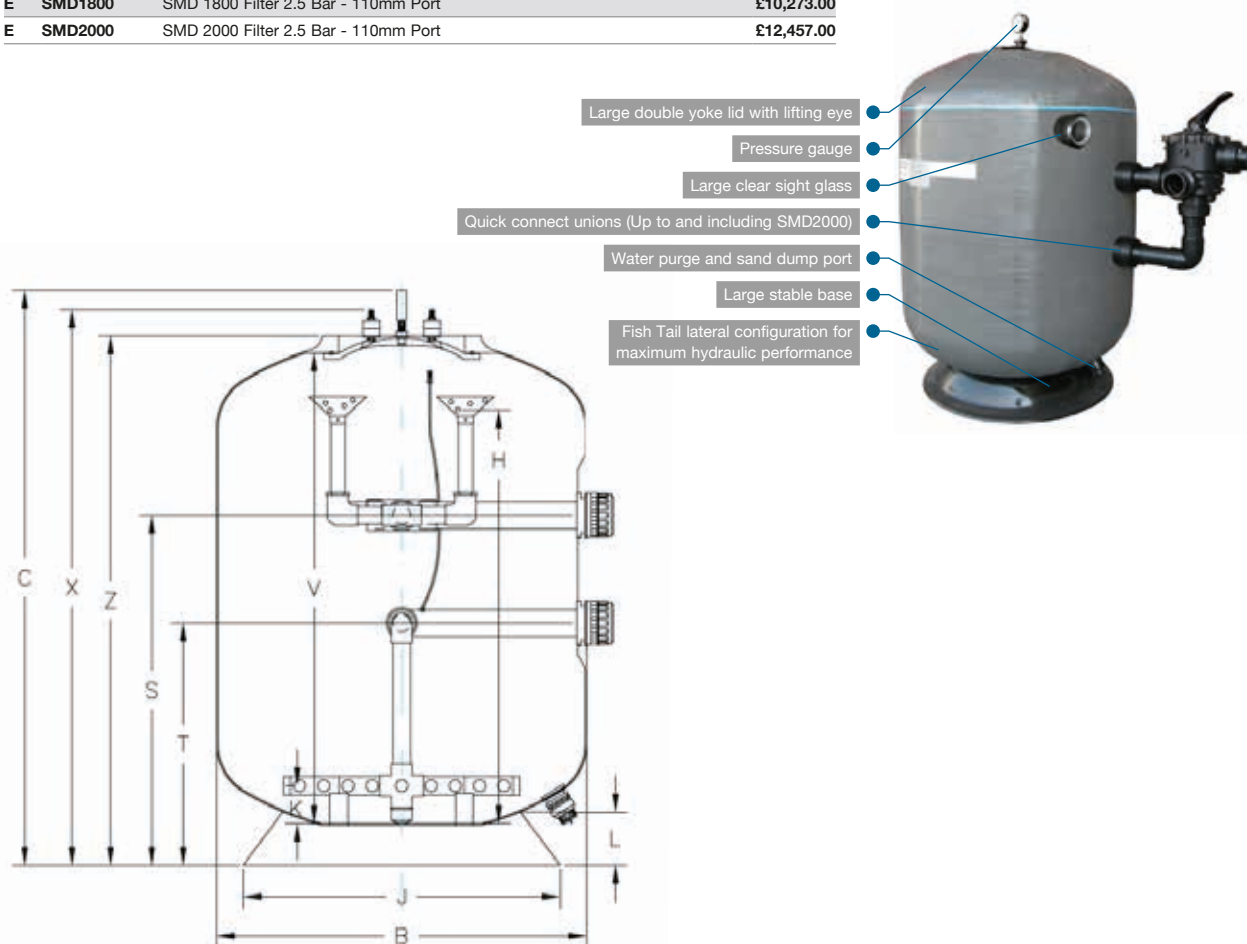
Dimensions (mm)
