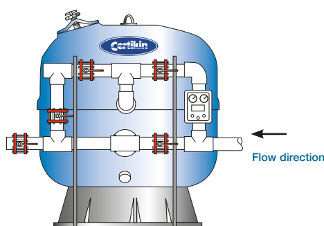
Single Filter 5 Valve Battery
