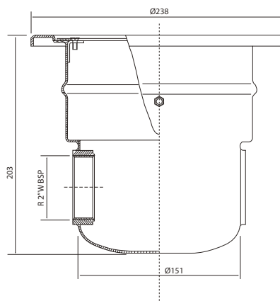
Stainless Main Drain - CKSS268 Flow Rate 13m³/hr
