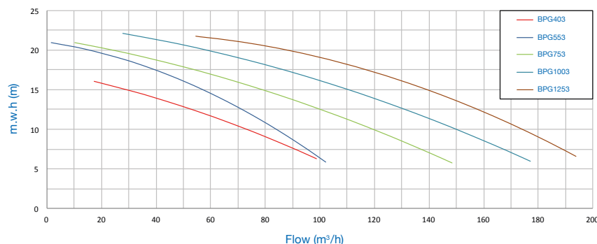
Characteristics curve
