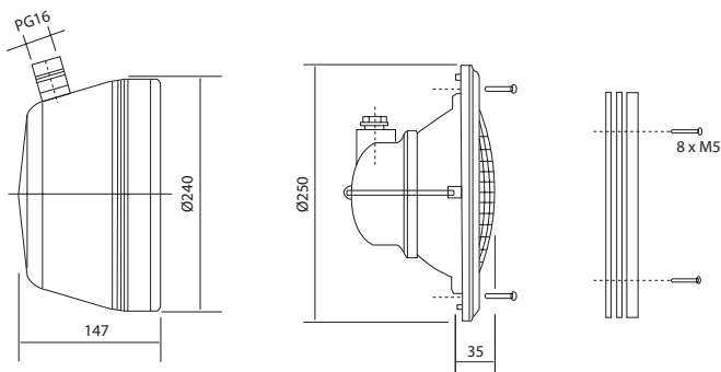
Stainless Steel Light - CKSS358
