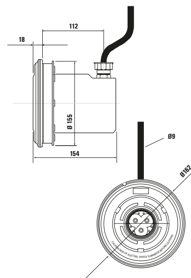
PLSC300CX-2 (multicoloured) PLSW300SCX (white)
