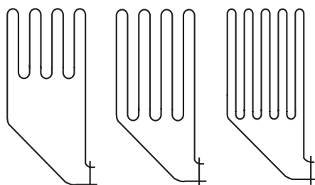
SPSH012 1500W 9kW x 6 10.5kW x 3 SPSH011 2000W 12kW - x 6 10.5kW - x3 SPSH010 200W 15kW x 6
