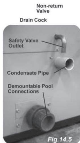
Condensing Pool Heater
